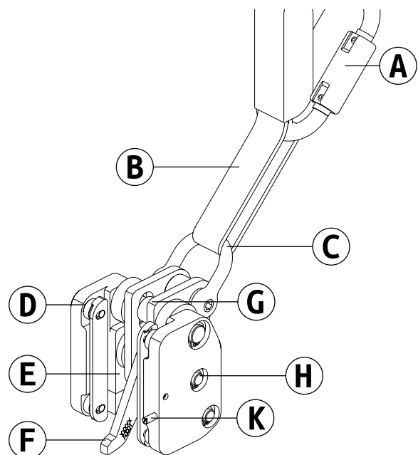
Fig. 14 GÜFA 5 safety-runner
