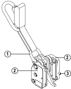
Fig. 16 guided type fall arrester (GÜFA 5)
