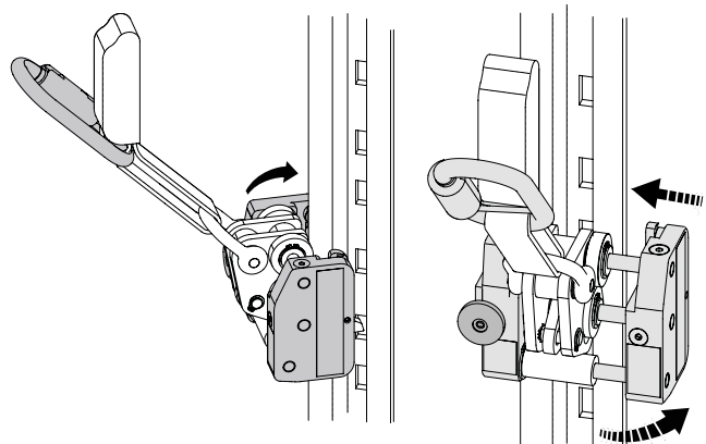
Fig. 20 Insert GÜFA Flexx into the arrester rail
